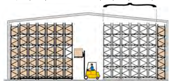
BITO PROmobile pallet racking
