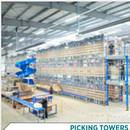
PICKING TOWERS
