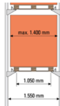
Bolted brackets for pallets with overhanging loads
