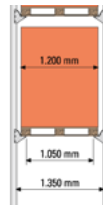
Hook-in brackets for pallets without overhanging loads
