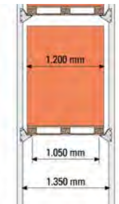
Hook-in brackets for pallets without overhanging loads
