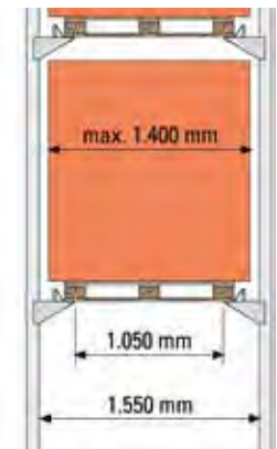
Bolted brackets for pallets with overhanging loads
